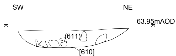
Section 48. SE facing section of pit [610].
